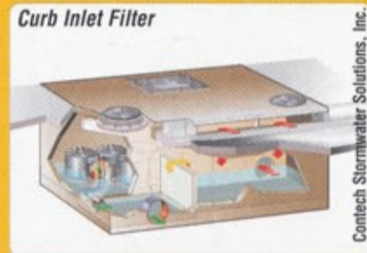
Curb Inlet Filter
