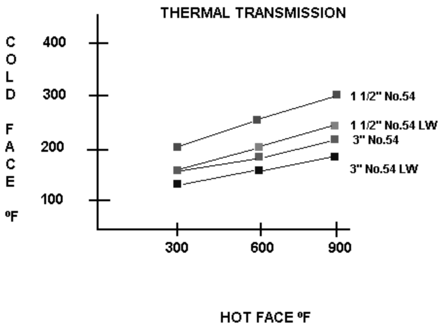
The Graph above illustrates the thermal transmission of No. 54 and 54 LW through various thicknesses.* Properties were obtained at an ambient temperature of 80°F and 10 mph wind velocity.
